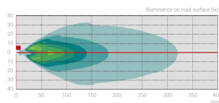
Isolux chart ECE 90 mm LED High Beam
