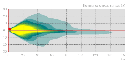
Isolux chart ECE LHD 90 mm LED Low Beam
